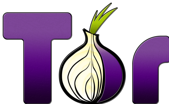
Figura 3.1: Tor logo
