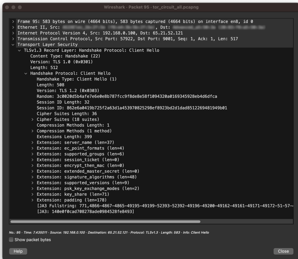
Figura 3.7: Client Hello
