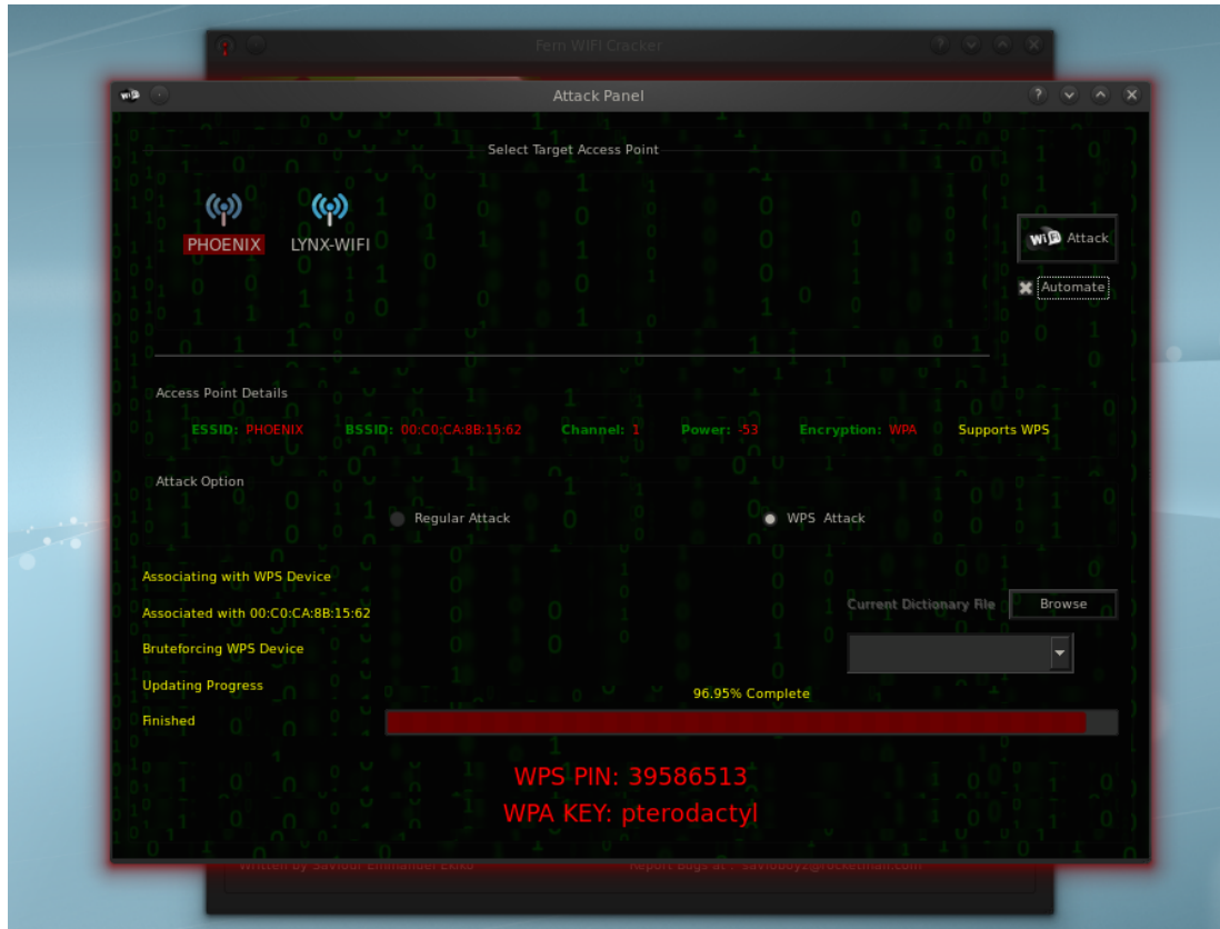
Figura 6.9: Fern-wifi-cracker attack
